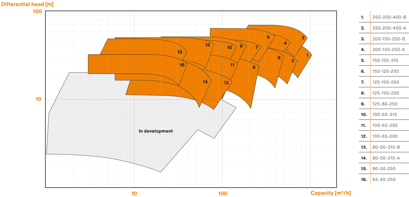
PERFORMANCE RANGE CHARTS 1450 MIN -1 (50 HZ 4-POLE)
