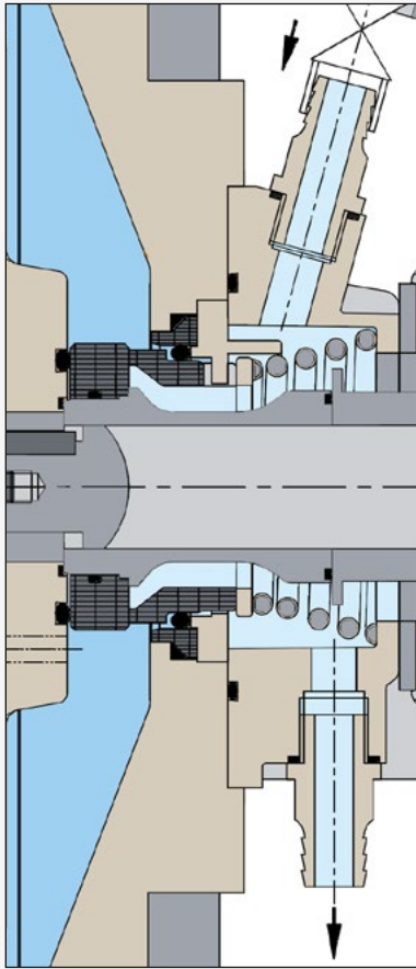
SPRING CHAMBER FLUSHING SYSTEM
