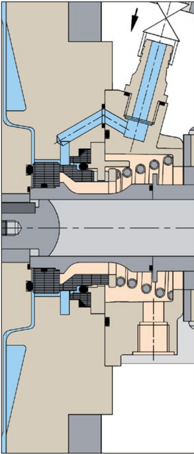
CONTINUOUS FLUSHING SYSTEM
