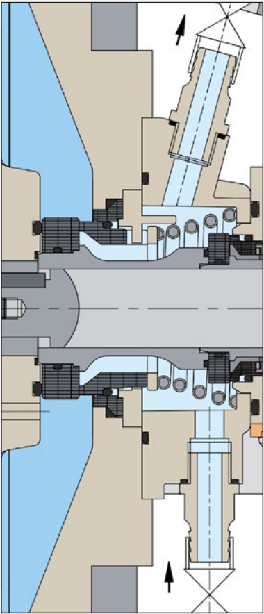
DOUBLE MECHANICAL SEAL
