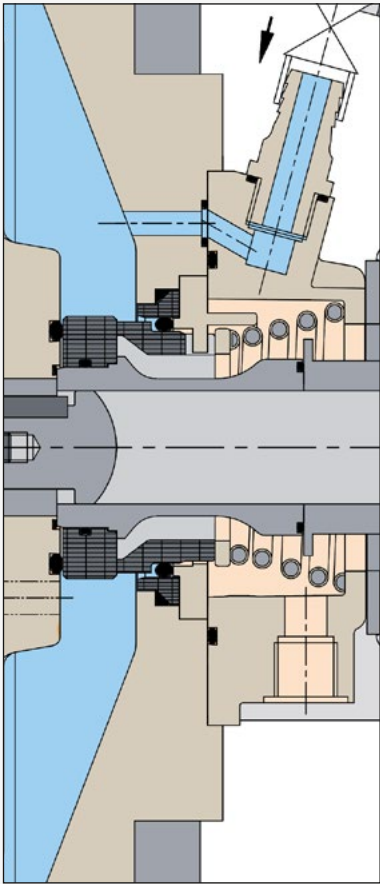
SHUTDOWN FLUSHING SYSTEM
